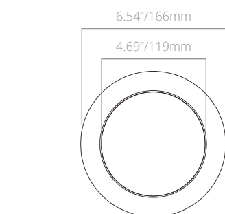
6" Trim Ring
